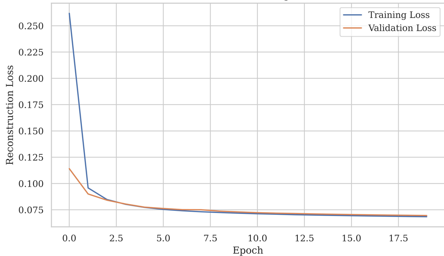
Convolutional Autoencoder: Training and Validation Loss
